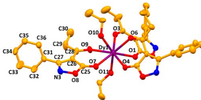
Figure 2. Perspective view of complex 1 . Thermal ellipsoids are drawn with 30% probability, and hydrogen atoms are omitted for clarity.
