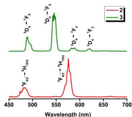
Figure 10. Triboluminescence (TL) spectra (uncorrected) of crystals of 2 and 3 recorded at 298 K. Vertical scale: arbitrary units.
