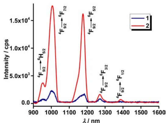
Figure 6. Corrected NIR emission spectra for \text{Dy}^{\text{III}} complexes 1 and 2 in the solid state at 298 K ( \lambda_{\text{ex}} = 320 nm).
